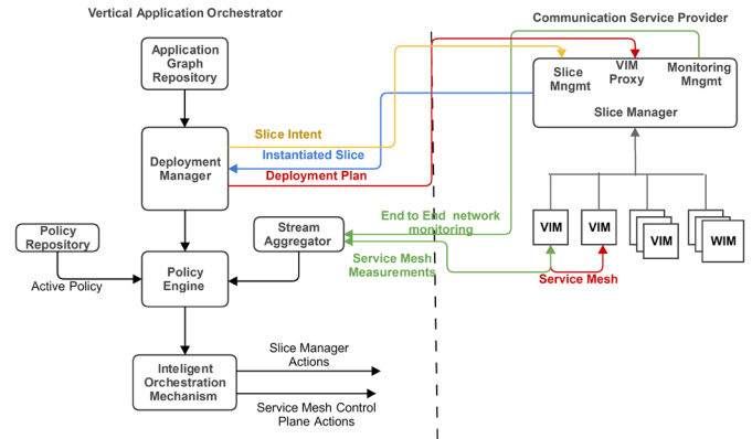
Fig. 3. Separation of concerns among orchestration domains.
