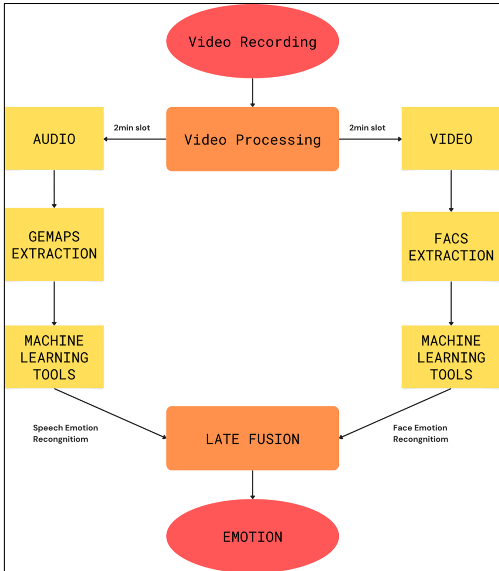
Figure 1: Our methodology
