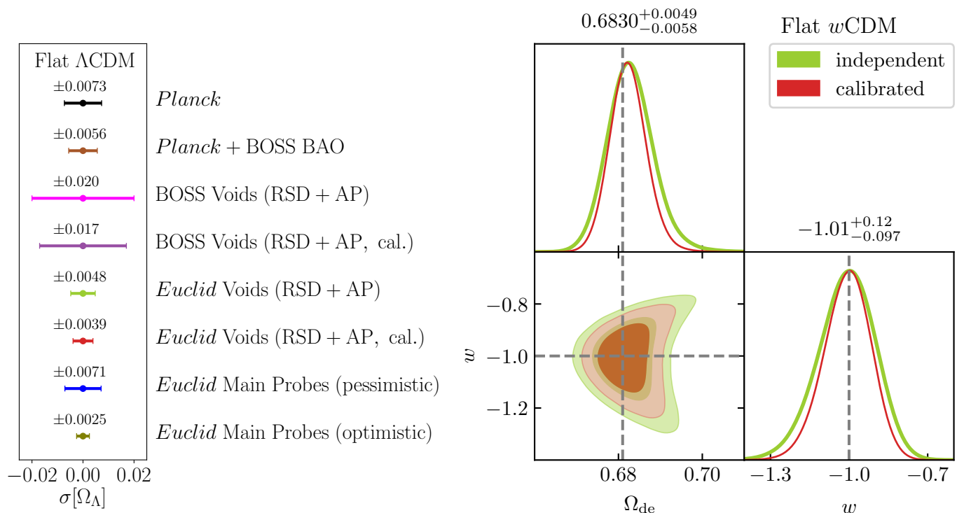
Fig. 7. Forecast for cosmological constraints on dark energy parameters. Left: Comparison of the constraining power on \Omega_\Lambda in a flat \Lambda CDM cosmology from Planck 2018 alone (Planck Collaboration et al. 2020) and when combined with BOSS BAO data (Alam et al. 2017). Below, constraints as obtained with BOSS voids via RSD and AP (Hamaus et al. 2020), as expected from Euclid voids (this work), and as expected from Euclid ’s main cosmological probes combined (Euclid Collaboration: Blanchard et al. 2020). Calibrated constraints from voids are indicated by the abbreviation “cal.” and the Euclid main probes distinguish between “optimistic” and “pessimistic” scenarios. Right: Predicted constraints from Euclid voids on dark energy content \Omega_{\text{de}} and its equation-of-state parameter w in a flat w CDM cosmology. Both the model-independent (green) and the calibrated results (red) are shown, dashed lines indicate the input cosmology. Mean parameter values and their 68% confidence intervals for the model-independent case are shown at the top of each panel.
