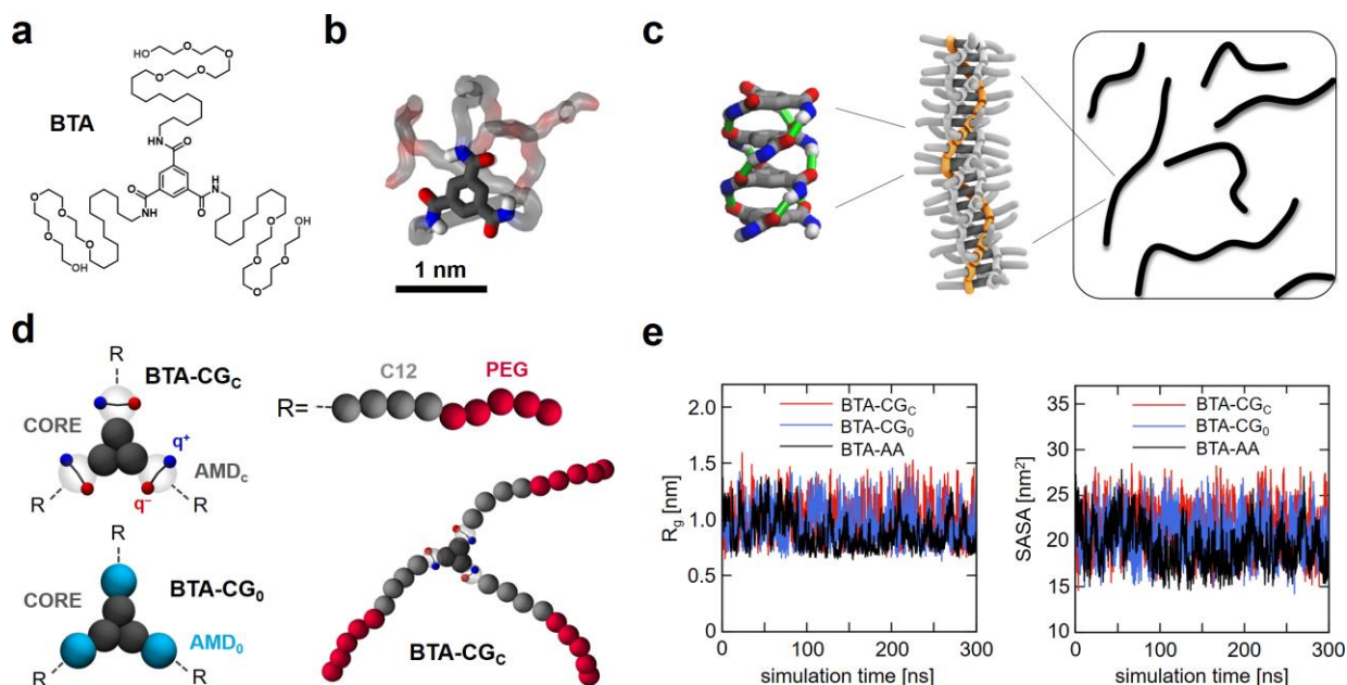
Figure 1. The reference water-soluble BTA monomer studied herein. (a) Chemical structure. (b) Equilibrated atomistic model for the BTA in water. 26,27 (c) 1D self-assembly through core-core stacking and threefold H-bonding between the BTA amides leading to fiber growth. (d) MARTINI-based CG models for the core and side chains of the BTA. BTA-CG c and BTA-CG 0 models differ in the description of the amides (with or without explicit description of inter-monomer H-bonding respectively). (e) Consistency of the radius of gyration ( R_g ) and SASA data at AA and CG level obtained from the MD simulations of a single BTA monomer in water.
