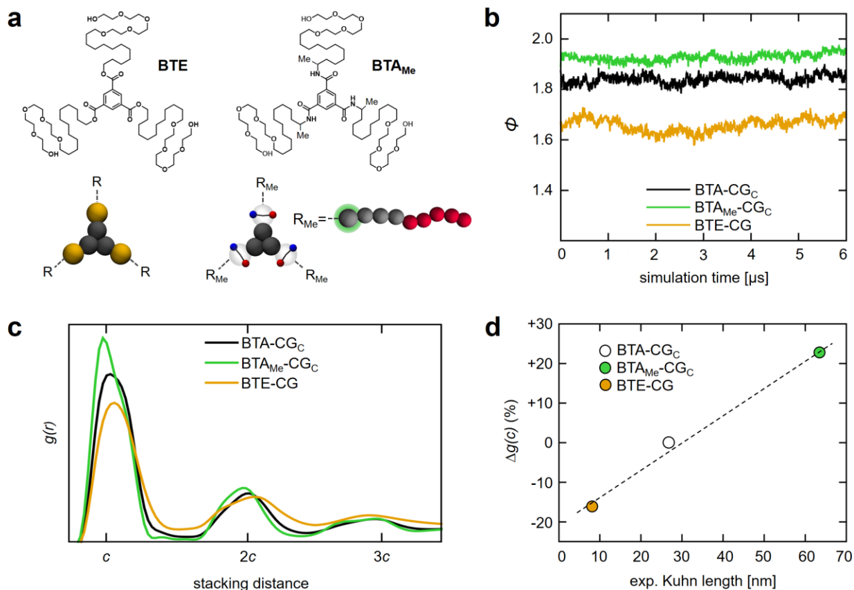
Figure 5. Transferability of the CG models and structure-property relationships. (a) Structure and CG models for the BTE and BTAMe monomer variants. (b) Order parameter \Phi as a function of time extracted from the CG-MD simulations of BTA-CG C , BTE-CG and BTAMe-CG C 480* infinite fiber models in water. (c) Radial distribution function g(r) of the cores of the monomers extracted from the equilibrated phase of the CG-MD simulations for the three systems. (d) Linear trend between the % variation of g(c) (the height of the first g(r) peak, relative to direct core-core stacking) calculated respect to the BTA-CG C system (reference and set to 0) and the experimental Kuhn length of the three different fibers. 26,27
