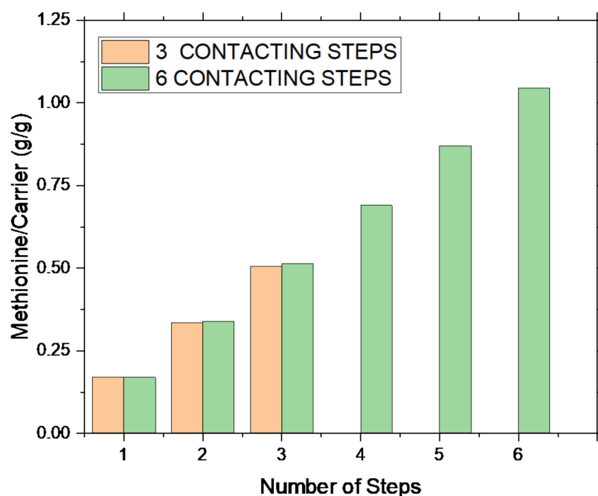
Figure 5. Methionine capture as a function of repeated three or six intercalation steps for the system MET–ADS.
