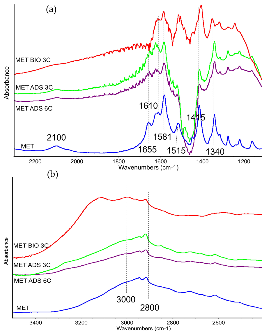
Figure 6. FTIR subtraction spectra (Adsorbene/BioKi + methionine) – (Adsorbene/BioKi) following multiple contacting tests: three steps and six steps. Pure methionine spectrum is also reported as reference: (a) low frequency region; (b) high-frequency region.
