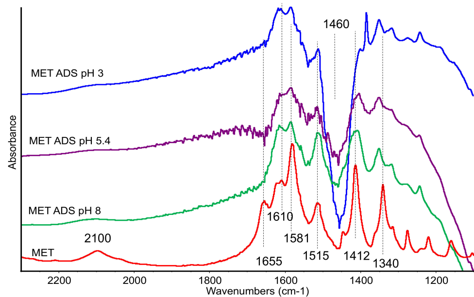
Figure 3. FTIR subtraction spectra (ADS + MET) – (ADS) at different pH. Pure methionine spectrum is also reported as reference.
