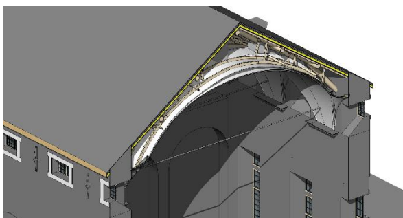
Figure 7 The Oratorio degli Uomini , one of the main wings to be renovated, BIM model (R. Babbetto). The design solution previews a new insulating layer under the roof.
