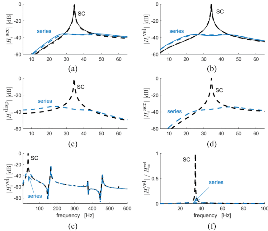
Figure 10. FRFs in terms of acceleration with an NC in series and \tilde{k}_i = 0.5948 (Test C), L^{\text{opt}} = 67.59 H, R^{\text{opt}} = 13.04 k \Omega (a), and FRFs in terms of mobility with an NC in series and \tilde{k}_i = 0.6734 (Test B), L^{\text{opt}} = 61.10 H, R^{\text{opt}} = 12.21 k \Omega (b). Experimental FRFs of plot (b) depicted in terms of dynamic compliance (c) and acceleration (d). Experimental FRFs of plot (b) on a wide frequency range (e), and in linear scale (f). Solid curves for the model expectations and dashed curves for the experiments.
