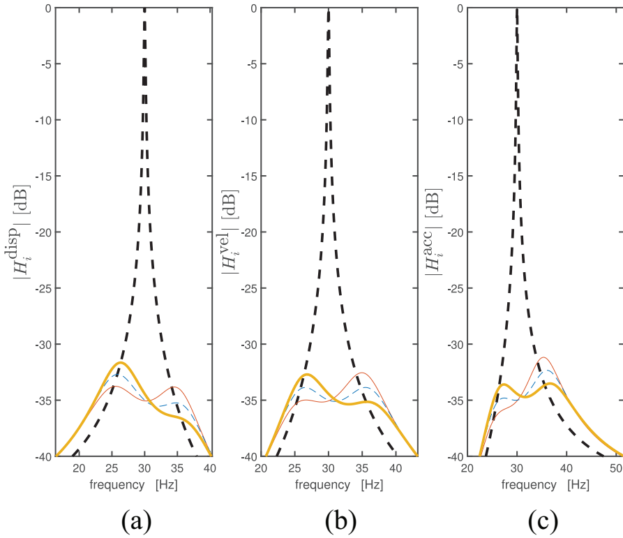
Figure 2. FRFs for a system with k_i = 0.3 , \tilde{k}_i = 0.4 , \xi_e = 0.3\% , \omega_i/(2\pi) = 30 Hz, NC connected in series, and L and R connected in series: (a) FRFs in terms of dynamic compliance (i.e. |H_i^{\text{disp}}| ), (b) FRFs in terms of mobility (i.e. |H_i^{\text{vel}}| ), and (c) FRFs in terms of accelerance (i.e. |H_i^{\text{acc}}| ). Thick dashed line for FRFs with the piezoelectric patch in SC (without NCs), thin solid line for FRFs with L and R set using the criteria found for the dynamic compliance optimisation, thin dashed line for FRFs with L and R set using the criteria found for the mobility optimisation, and thick solid line for FRFs with L and R set using the criteria found for the accelerance optimisation.
