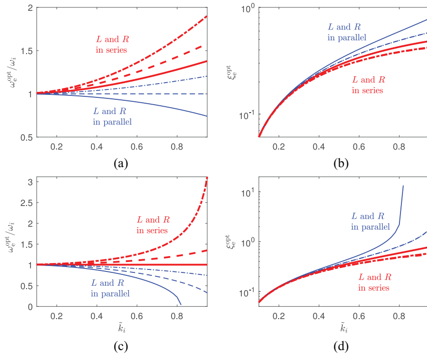
Figure 3. Trends of \omega_e^{opt} (normalised over \omega_i ) and \xi_{sc}^{opt} as a function of \tilde{k}_i for a system with k_i = 0.1 : NC in parallel for plots (a) and (b), and NC in series for plots (c) and (d). Red thick lines for R and L connected in series and blue thin lines for R and L connected in parallel. Solid line for control in displacement, dashed line for velocity and dash-dotted line for acceleration.
