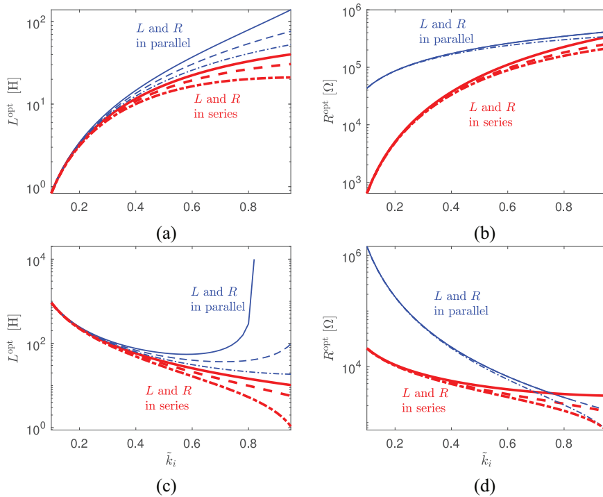
Figure 4. Trends of L^{opt} and R^{opt} as a function of \tilde{k}_i for a system with k_i = 0.1 : NC in parallel with \omega_i/(2\pi) = 1000 Hz for plots (a) and (b), and NC in series with \omega_i/(2\pi) = 30 Hz for plots (c) and (d). Red thick lines for R and L connected in series and blue thin lines for R and L connected in parallel. Solid line for control in displacement, dashed line for velocity and dash-dotted line for acceleration.
