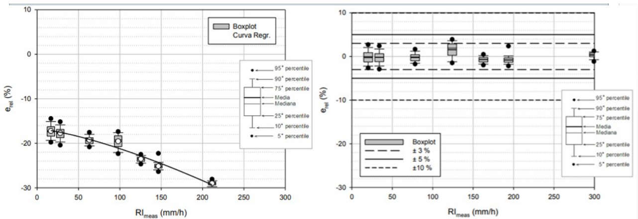
Figura 2. Relative errors (in %) related to ISCO 674 Rain Gauge without correction (left) and with correction (right) obtained using the intertip algorithm.
