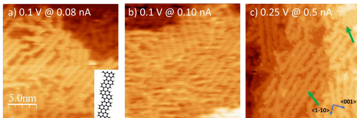
Figure 3. STM images showing overviews of the Ag(110) surface covered by a sub-monolayer of GNRs and subject to different treatments: a) pristine GNRs; b) same as a) after exposure to O_2 at room temperature; c) same as a) after exposure to O_2 at 300 °C. The nominal O_2 dose is always 900 L ( \sim 4500 L when considering the doser enhancement factor). The green arrows in c) point to additional features forming both in-between the GNRs and on bare Ag(110) areas.
