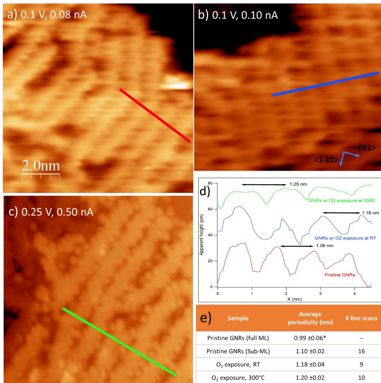
Figure 6. Close up images of the three preparations in Figure 3 with corresponding line scans indicating the periodicity of the GNRs. A: Pristine GNRs; b) same as a) after exposure to O 2 at RT; c) same as a) after exposure to O 2 at 300 °C. In this preparation the small features in-between the GNRs are evident. d) Line scans cut along the paths marked in panels a-c) showing that the separation between adjacent GNRs increases after O 2 exposure. e) Table summarizing the average separation between GNRs in ordered arrays, together with the number of line scans considered for each preparation (corresponding to the number of GNRs arrays considered). Values are given with their standard error. Data indicated with * are taken from ref. 12
