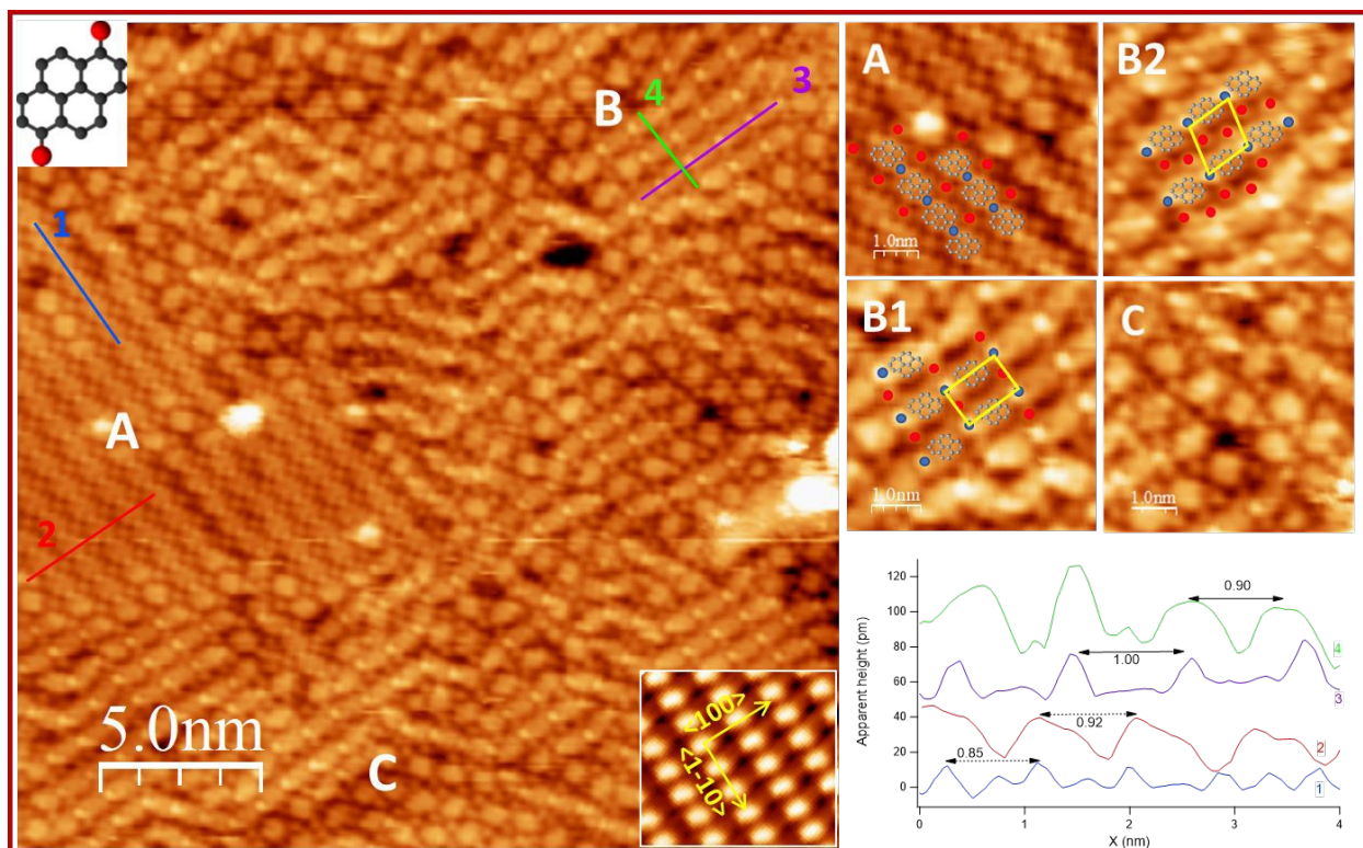
Figure 1. Left: STM image ( V=-150 meV, I=0.3 nA) showing the co-existence of three different self-assembled structures (labelled as A, B, C) upon deposition of a sub-monolayer of DBP on Ag(110) at RT. Top and bottom insets report, respectively, the molecular structure of DBP and the atomically resolved image of clean Ag(110) from which the high symmetry directions (marked by arrows) are determined (image size: 1.8 \times 1.6 nm 2 ). Top right: enlarged image of each domain (either from the area in the overview or from neighbouring areas). Among B domains, it is possible to distinguish rectangular (B1) and rhomboidal unit cells (B2). Empirical models deduced from the periodicities of the self-assembled structures and from XPS results are superimposed to the STM image for structures A, B1 and B2 (grey: de-brominated pyrene units; blue: Ag adatoms; red: Br atoms). Bottom right: line scans cut across the paths marked in the overview for structures A and B1 (follow colour code). Line scans drawn along and across the rows of structure B2 are not reported since they do not differ significantly from those of B1. The higher and sharper features in traces 1 and 3 correspond to the Ag atoms within the organometallic chains.
