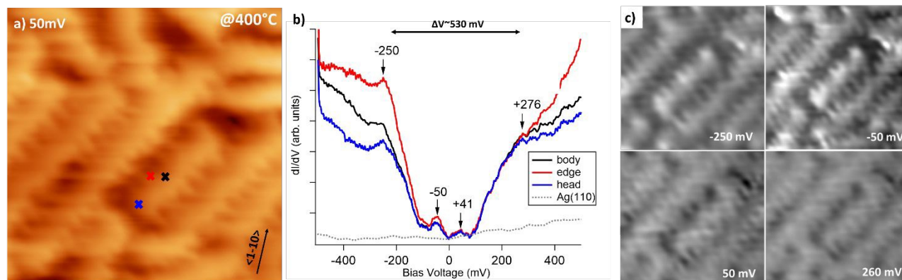
Figure 4. STS and dI/dV map of pristine GNRs in the bias range from -500 mV to 500 mV. a) Topographical image (Image size: 7.0 \times 7.0 nm 2 , V=50 mV, I=0.02 nA); crosses indicate the sites where point spectra were recorded. b) Differential conductance spectra recorded at the points marked in a). The corresponding spectrum recorded on clean Ag(110) is reported for comparison. A band gap of \sim 530 meV was observed throughout the GNR. Localized states at -50 meV and +41 meV are present within the gap. Such values were measured reproducibly for 3-5 nm long GNRs; it is out of the scope of this work to determine a possible length dependence of the energy gap. c) dI/dV maps taken at selected bias voltage suggested by the STS spectra.
