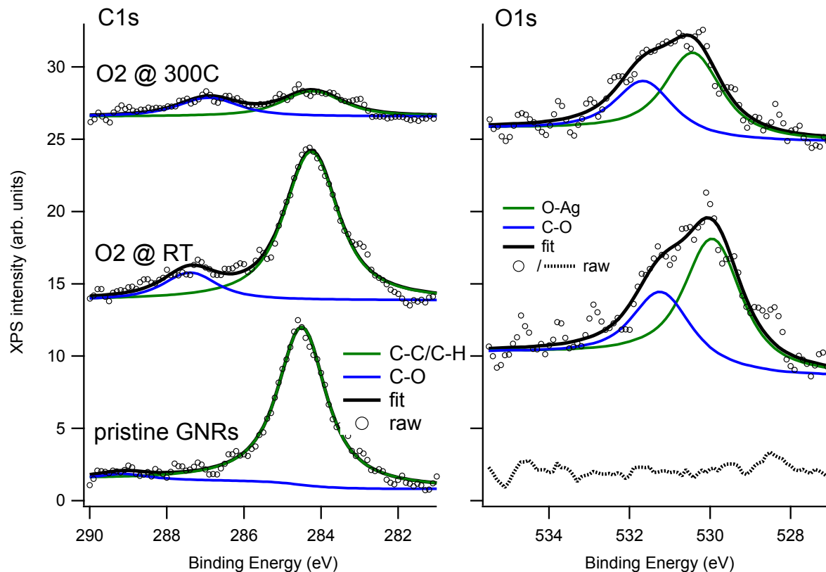
Figure 5. XPS spectra of the C 1s (left) and O 1s (right) regions recorded on the GNRs/Ag(110) surface before and after O 2 exposure.
