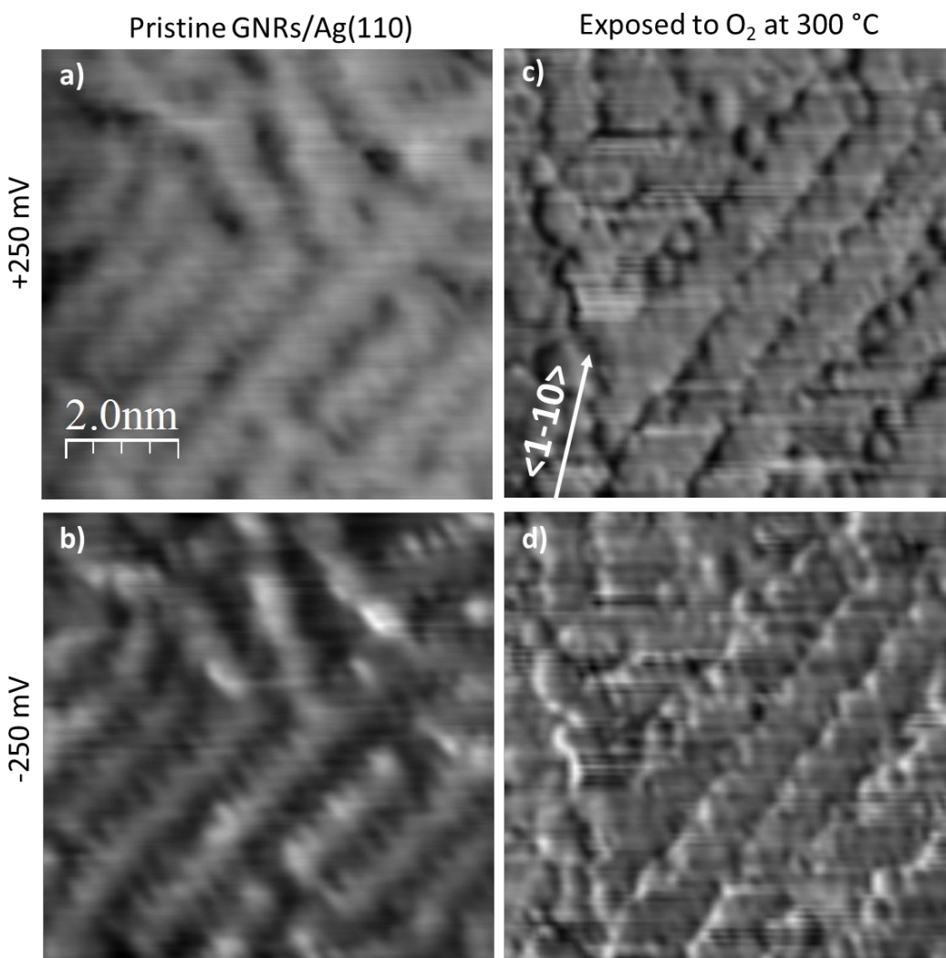
Figure 7. Comparison of the dI/dV maps of GNRs pristine and after exposure to oxygen at 300 °C. Bias voltages corresponding to the edges of the energy gap measured for the pristine sample are presented. The corresponding topographical images are those of Figures 4a and 5c. Z-scale is the same for all images.
