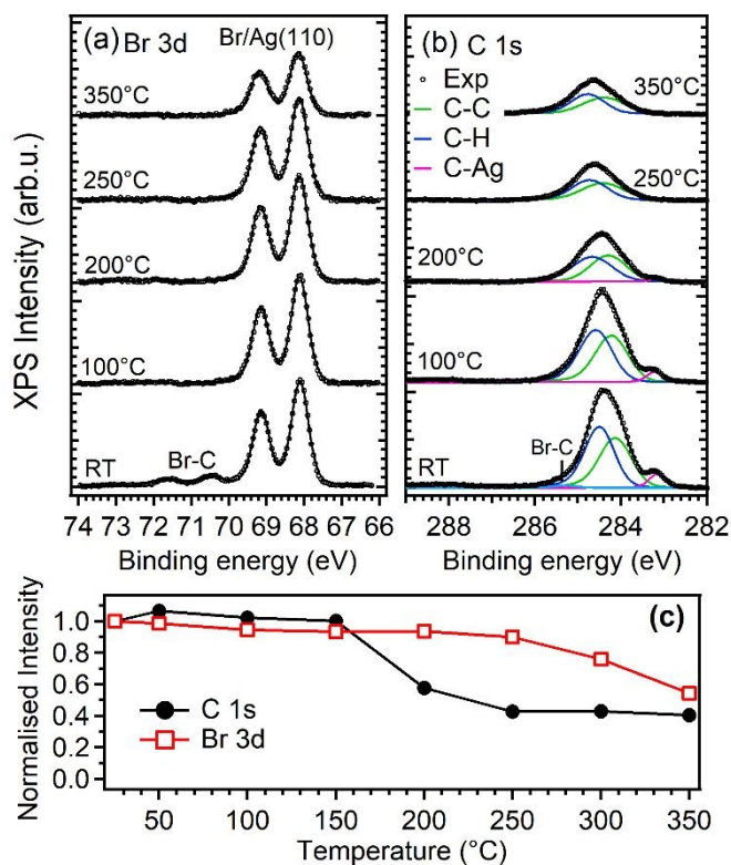
Figure 2. (a) Br 3d and (b) C 1s core level spectra of 0.6 ML of DBP deposited on Ag(110) at RT and after annealing the sample to the indicated temperature for 5 minutes. (c) Normalized integrated intensity of Br 3d and C 1s peaks as a function of temperature. The intensities are normalized to the peak areas measured after the deposition.
