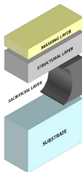
Figure 9. Three-D sketch of the proposed device.
