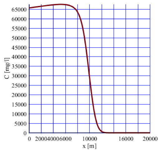
Figure 3. Concentration profile at t = 5110 [d].
