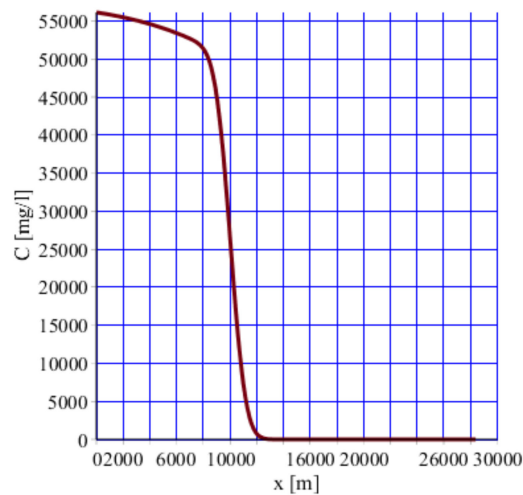
Figure 5. Concentration profile at t = 5110 [d].
