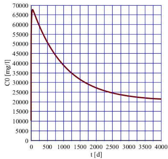
Figure 2. Concentration profile at x = 0 .
