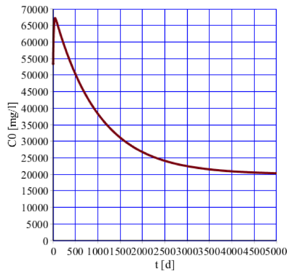
Figure 4. Concentration profile at x = 0 .
