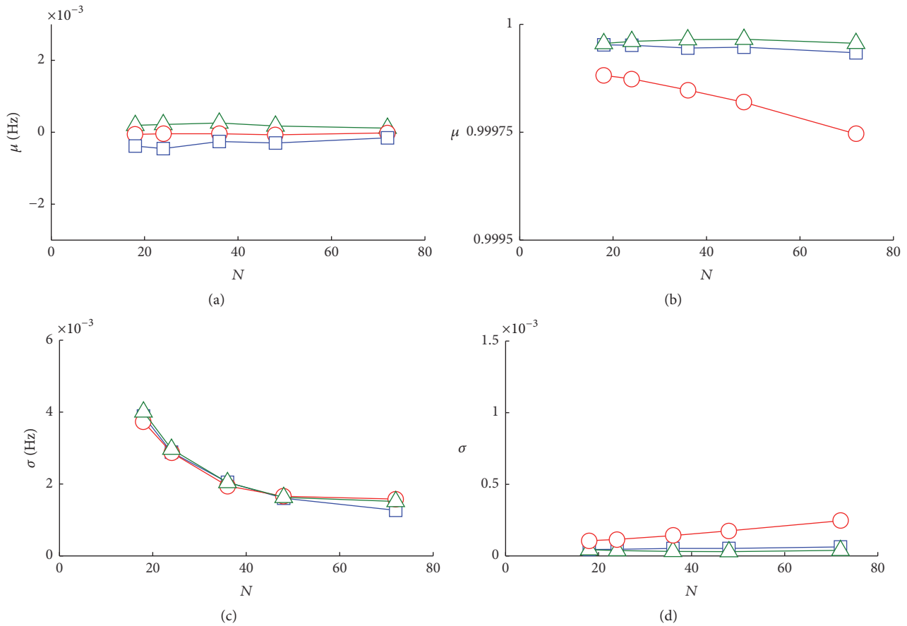
FIGURE 6: Results of the MCMC simulations for FDD as function of N ( R = 5 mHz): mean value of the error for the eigenfrequency estimation (a), mean value of the MAC (b), \sigma of the error for the eigenfrequency estimation (c), and \sigma for the MAC (d). Curves with squares ( \square ) for the first mode, with circles ( \circ ) for the second mode, and with triangles ( \triangle ) for the third mode.
