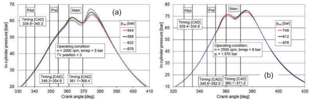
Figure 4. Influence of rail pressure on in-cylinder pressure diagrams.
