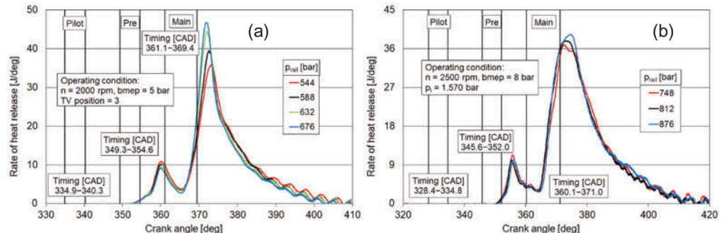
Figure 6. Influence of rail pressure on heat release rates.
