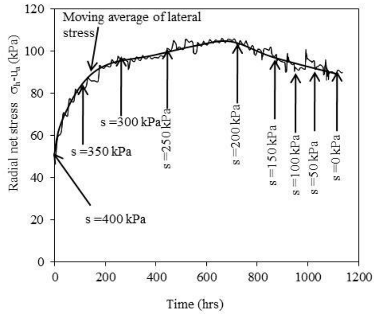
Figure 5 Variation of radial net stress during decrease in suction 50 kPa step
