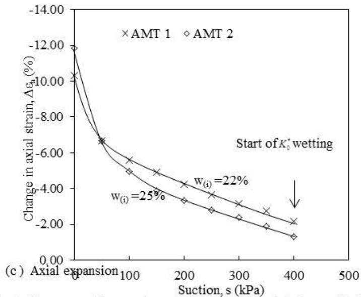
Figure 13 Effect of compaction water content on water intake, radial net stress and axial swelling during \kappa_s^* wetting (AMT)
