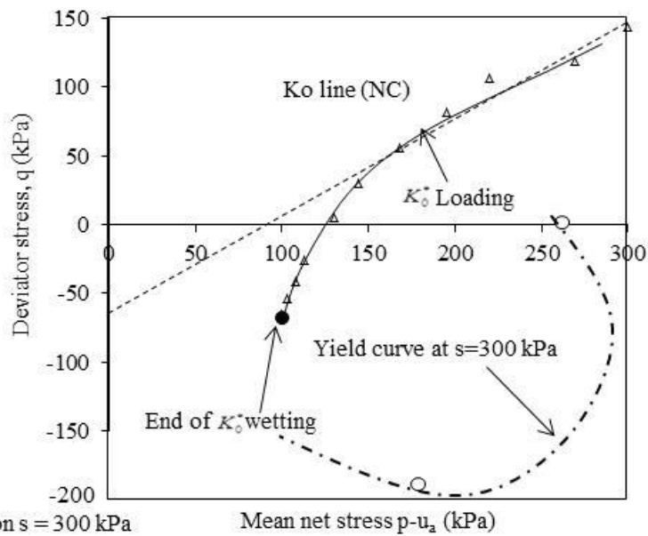
Figure 16 Stress path during K_0^* loading and yield locus at different suctions (KC)
