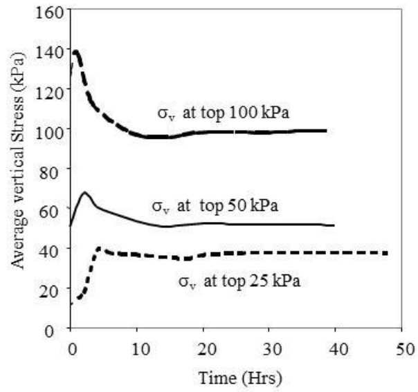
Figure 1 Wetting of compacted kaolin in Rowe Cell under various vertical pressures
