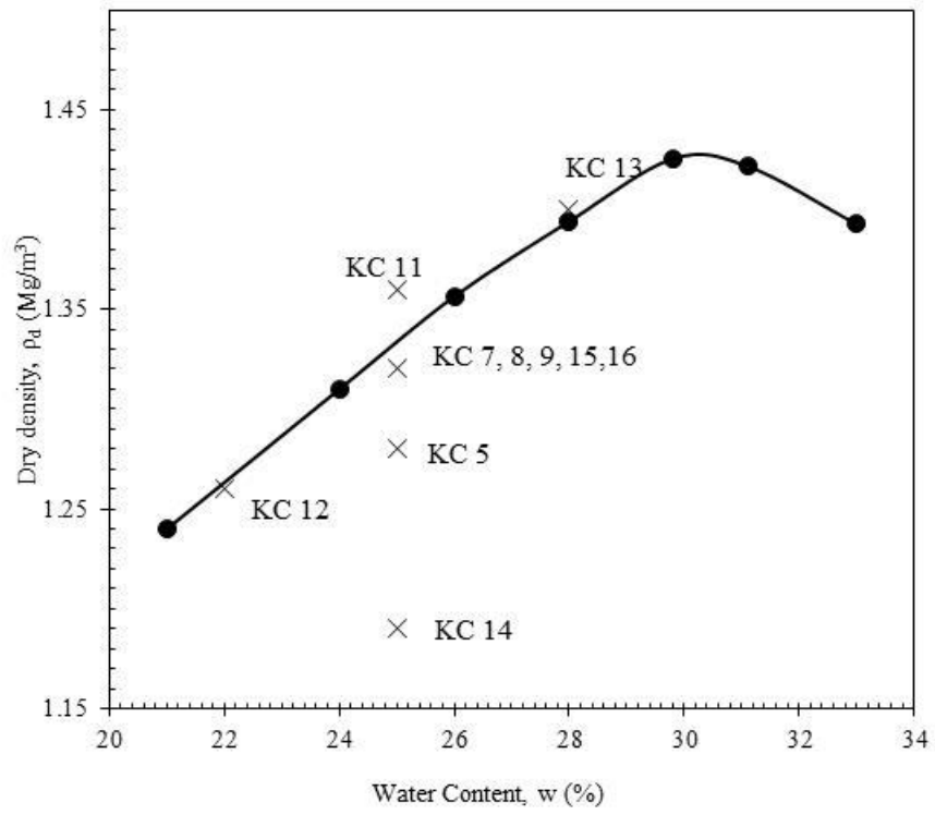
Figure 2 Proctor compaction curve: kaolin clay
