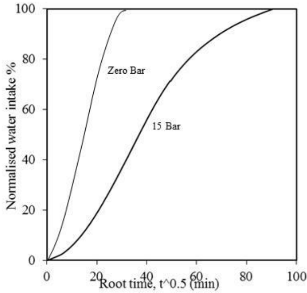
(a) Effect of air entry ceramic filter on the water flow into the sample
