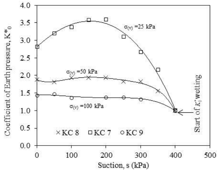
(b) K^*_0
