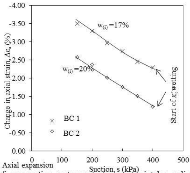
Figure 12 Effect of compaction water content on water intake, radial net stress and axial swelling during \kappa_s^* wetting (BC)
