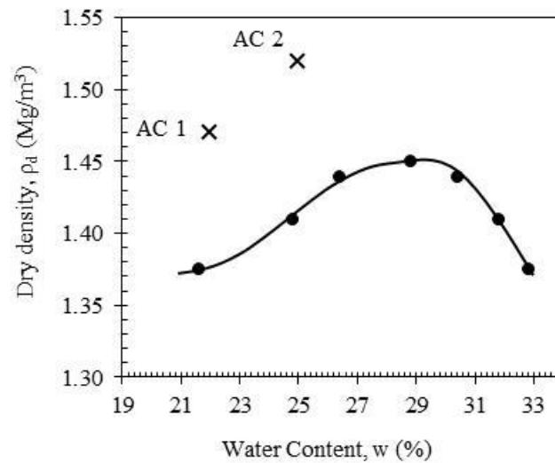
Figure 3 Proctor compaction: London Clay, Belfast Clay and Amphthil Clay
