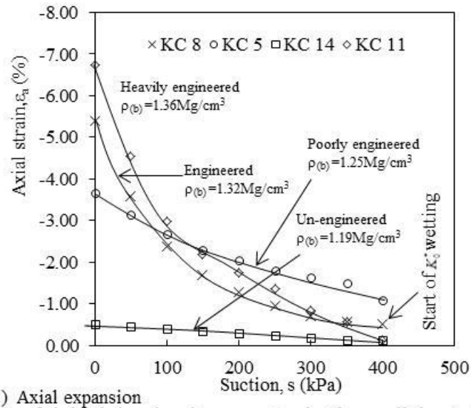
Figure 9 Effect of initial dry density on water intake, radial net stress and axial swelling during \kappa_s^0 wetting (KC)
