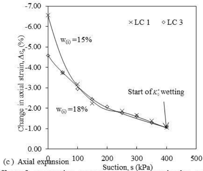
Figure 11 Effect of compaction water content on water intake, radial net stress and axial swelling during \kappa'_0 wetting (LC)
