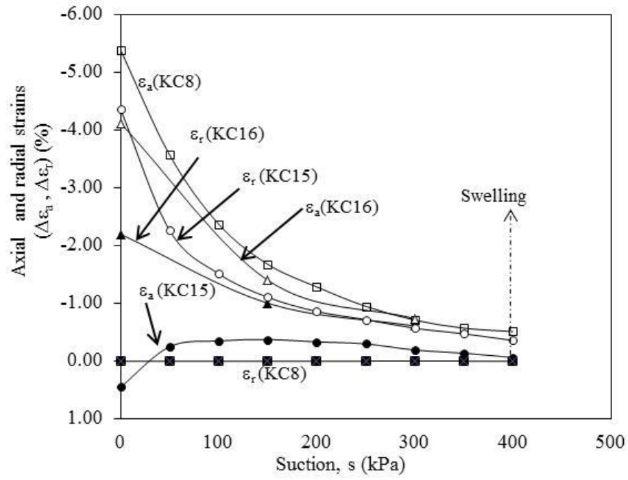
Figure 6 Swelling/collapse of compacted kaolin
