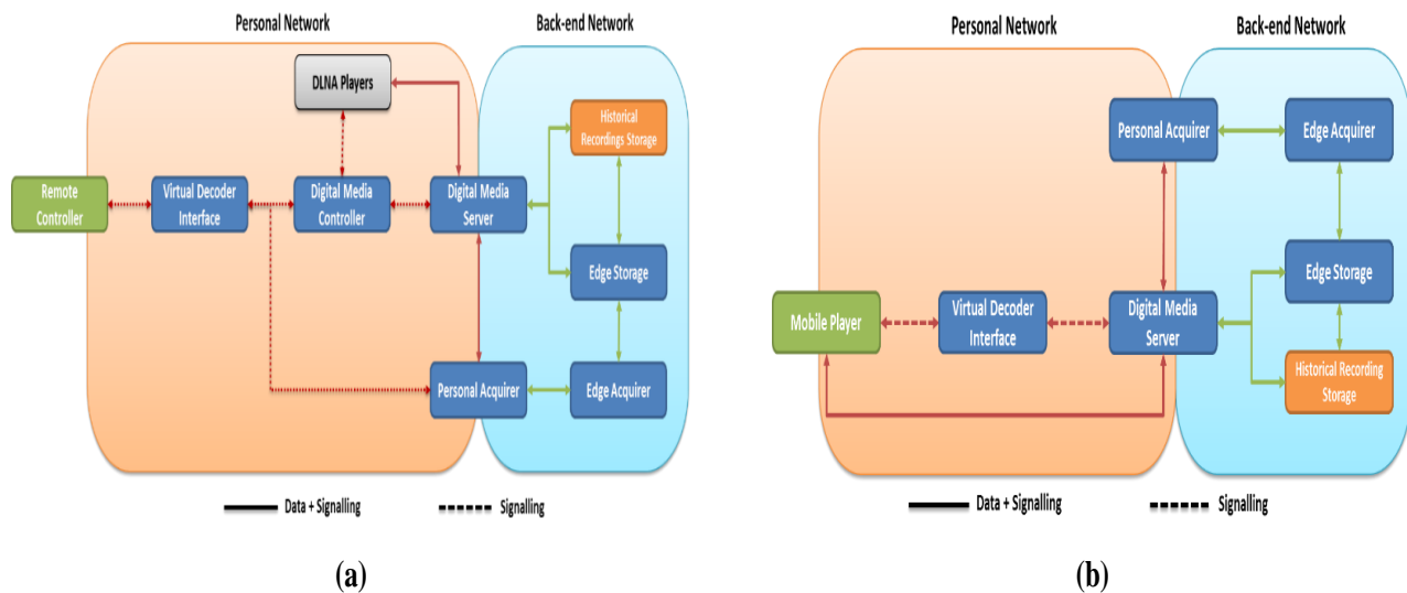
Figure 7. Service chains for live multimedia content view on (a) smart TV and (b) mobile device.
