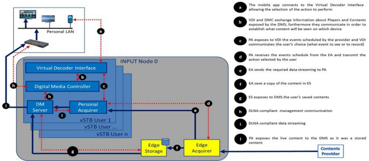
Figure 6. Data and signaling messages exchanged among the vSTB core elements and the physical devices attached to the user's residential local area network.
