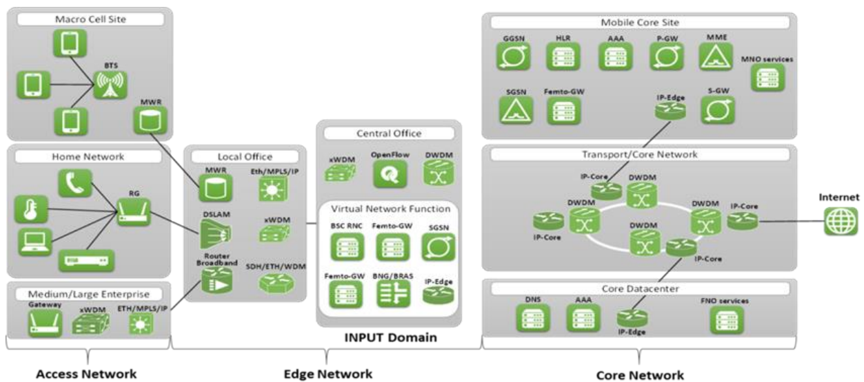
Figure 2. IP Network architecture according to the SDN/NFV paradigm of the INPUT project.
