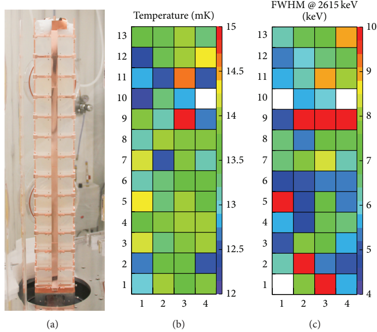
FIGURE 4: (a) The CUORE-0 tower inside a glove box during its assembly. (b) Base temperatures of the functioning CUORE-0 crystals, as calculated from the measured resistances of their thermistors in conjunction with R_0 and T_0 values previously determined in thermistor characterization studies (see Section 2). It should be mentioned that there is good evidence that a thermistor’s R - T behavior can be modified by mechanical stresses caused by its glue-spot connections to the crystal, and this effect could be responsible in part for the seemingly erratic distribution of detector temperatures. (c) Energy resolution (FWHM) of each detector channel, determined from calibrations performed regularly during March–September 2013. The mean energy resolution in the calibration data is 6.8 keV, and the median is 6.0 keV.
