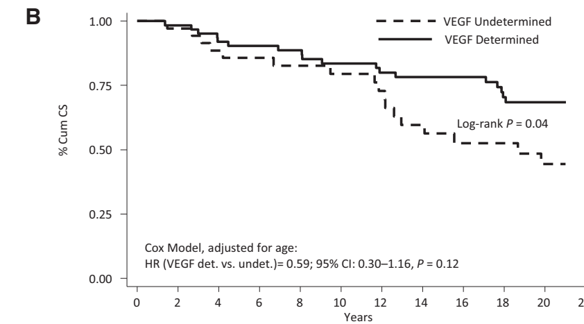
Figure 1. Kaplan-Meier OS (A), CS (B), and BCS (C) according to VEGF determination (undetermined, dotted line; determined, continuous line). HRs from a Cox proportional hazards model adjusted for age are provided.
