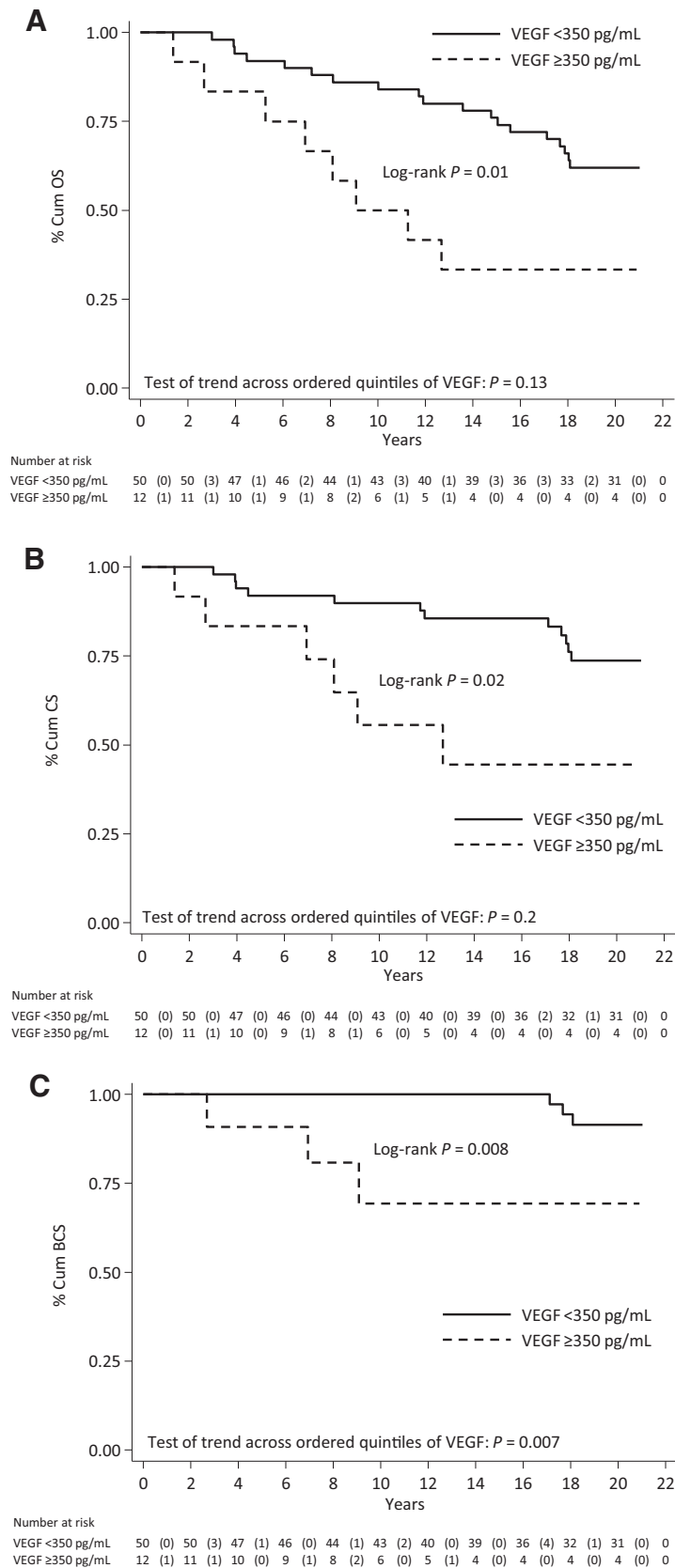
Figure 3. Kaplan-Meier OS (A), CS (B), and BCS (C) curves according to VEGF values at baseline (below vs. above or equal the top quintile, i.e., 350 pg/mL). P values for test for trend across ordered quintiles of VEGF are provided.
