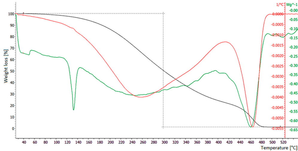
Figure 6. TG analysis of a PP sample. Black line: TGA (weight loss); red line: first derivative of the TGA; green line: DSC (differential scanning calorimetry).
