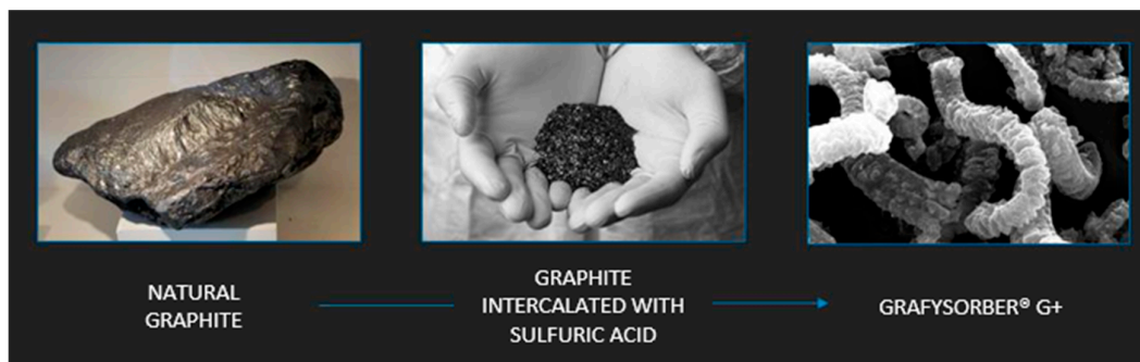
Figure 1. Production process of Grafysorber® G+.
