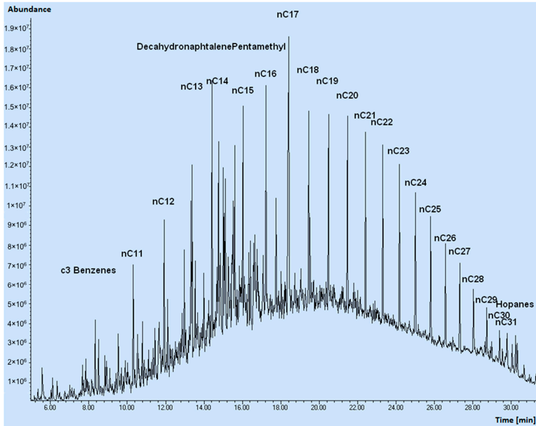
Figure 3. Total ion current chromatogram (GC-MS analysis) of the oil.
