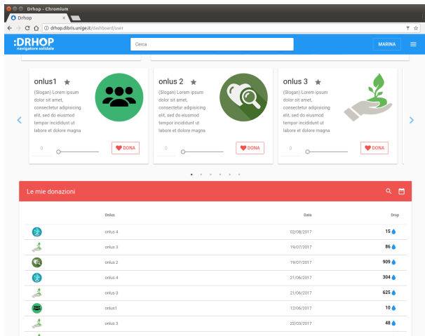
Figure 4: DONATE dashboard.
