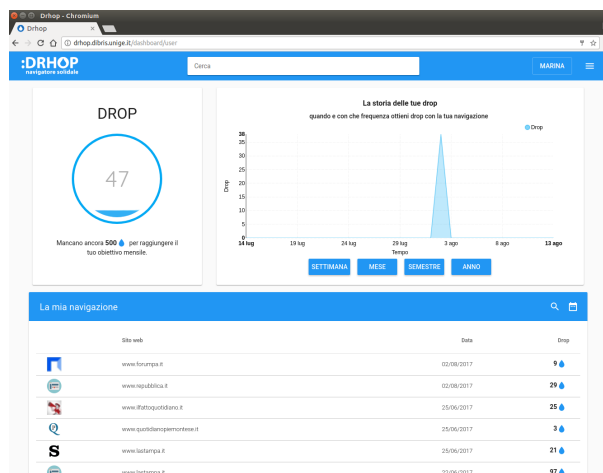
Figure 3: DROP dashboard.
