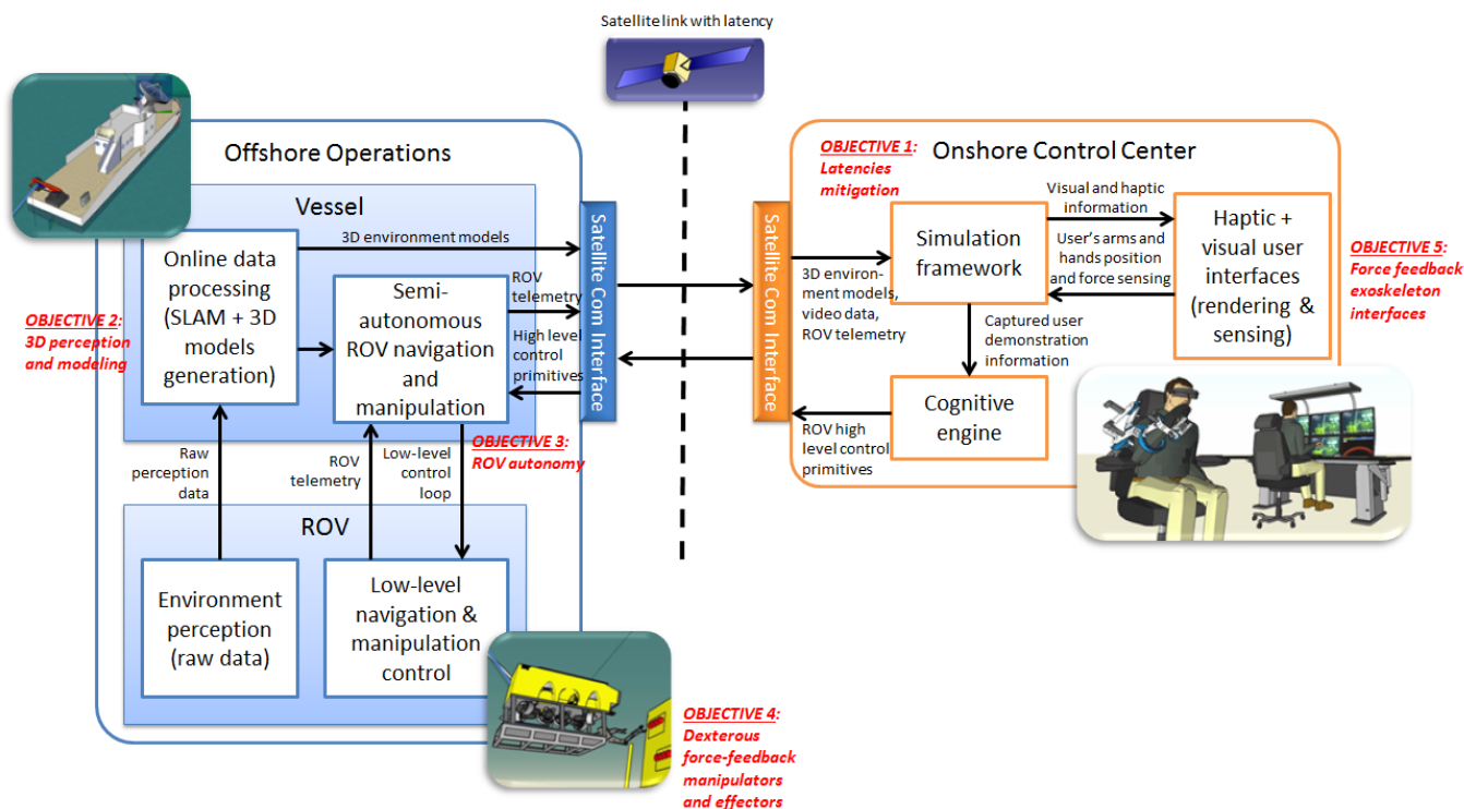
Fig. 1. DexROV functional architecture
