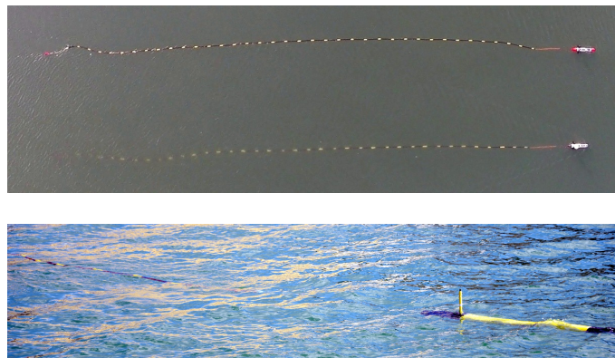
Fig. 1. Preliminary tests: MEDSUA (top) and Folaga (bottom) vehicles towing streamers.
