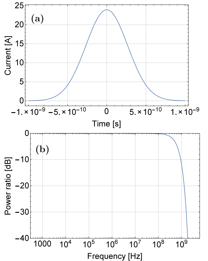
Figure 2. Instantaneous current of bunches of 10^{11} protons having a Gaussian longitudinal profile with \sigma = 8 cm (a), and the corresponding power spectrum, which is its Fourier transform (b).
