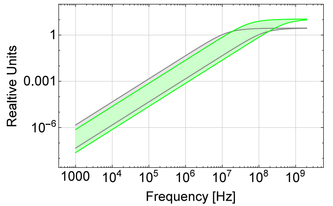
Figure 4. Ratio of expected surface resistances of Tl-1223 and Cu at 1.06 T (gray band), and at 16 T (green band). The bands correspond to the range of critical currents mentioned in the text.
