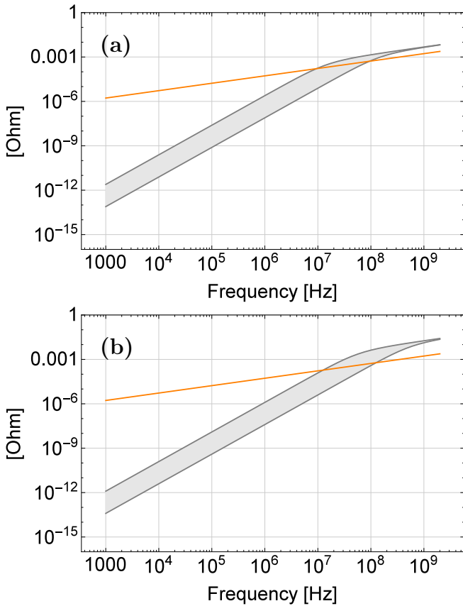
Figure 3. Predicted surface resistance at 50 K of Tl-1223 (gray band) compared to Cu (orange) at 1.06 T (a), and at 16 T (b). The band corresponds to the range of critical currents mentioned in the text.
