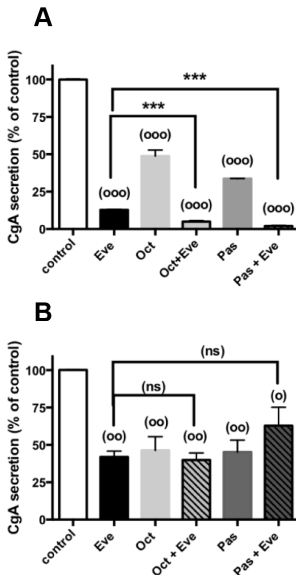
Figure 4: CgA secretion in combined treatments of everolimus with SSAs. Primary culture cells from (A) one pNET (n°4), (B) 10 pNETs (n° 3,6-8,10,11,15-17,19) were incubated for 72h in the absence (vehicle) or in the presence of 1nM everolimus (Eve), or 1nM octreotide (Oct), or 1nM pasireotide (Pas) alone (diluted in vehicle) or in the presence of everolimus and octreotide or everolimus and pasireotide as indicated in the figure. CgA secretion was determined as described in patients and methods. Results are expressed as mean \pm SEM ((A) n=1; (B) n=10) in percent of control. Each assay was performed in triplicate. (°) p<0.05; (°°) p<0.01 (°°°) p<0.001 versus control ; (***) p<0.001, (ns) not significant.
