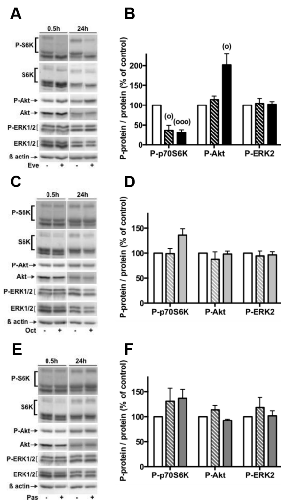
Figure 5: Effects of everolimus and the SSAs single treatments on the activity of the PI3K/Akt and MAPKinase ERK1/2 pathways. Primary culture cells from pNETs were incubated 30 min (3 pNETs) or 24h in the absence ( vehicle) or in the presence of 1nM everolimus (Eve) (7 pNETs) (A, B) or 1nM octreotide (Oct) (5 pNETs) (C, D) or 1nM pasireotide (Pas) (5 pNETs) (E, F). The phosphorylated levels of p70S6K, Akt and ERK1/2 were analyzed by using western blotting as described in patients and methods. Representative immunoblots are given in (A), (C), (E). Means \pm SEM in percent of control are given in (B), (D), (F) ((B) n=7 ; (D,F) n=5 ). Control condition (white bars), 30min treatment (hatched bars), 24h treatment (black and grey bars). (°) p<0.05 , (°°°) p<0.001 versus control.
