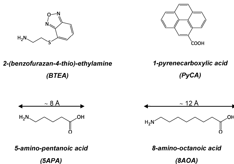
Scheme 1. Chemical formulas of the fluorescent probes (top) and alkyl spacers (bottom) employed in the synthesis of the core-shell metal nanohybrids.
