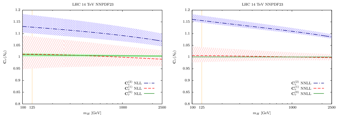
Figure 4. The ratio functions \mathbf{C}_r^{(i)}(N_0(\tau), M^2, \mu_s^2) eqs. (2.31, 2.36, 2.40), computed at NLL (left) and NNLL (right) as a function of the saddle point N_0(\tau) , and plotted versus the Higgs mass m_H . All settings are the same as in figure 2. The curves shown are, from top to bottom, \mathbf{C}_r^{(2)} , \mathbf{C}_r^{(1)} , and \mathbf{C}_r^{(0)} . In each case, the edges of the band correspond to the two different choices for \mu_s from refs. [6, 9, 19], and the central curve is their average.
