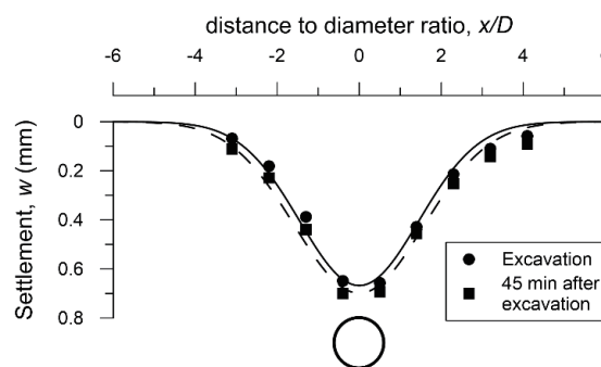
Fig. 4. Surface settlements obtained from centrifuge test.
