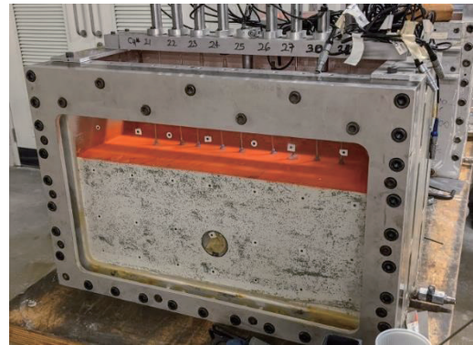
Fig. 2. Completed centrifuge model.
