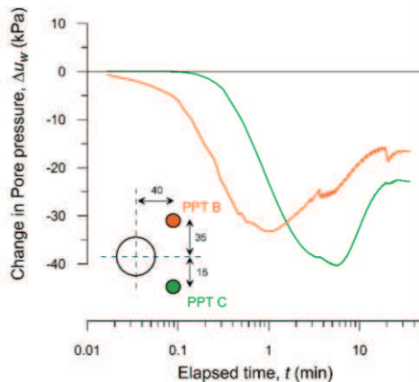
Fig. 5. Pore pressure changes post-excavation in Test 2.
