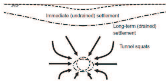
Fig. 1. Tunnelling-induced ground movements (Mair, 2008).
