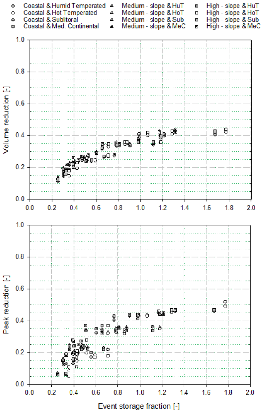
Figure 1. Volume and peak reduction indexes plotted versus the event storage fraction simulated for the three drainage network catchment typologies (Coastal, Medium-slope; High-Slope) according to the four precipitation regimes (Humid temperated, Hot temperated, Sublitoral and Mediterranean continental).
