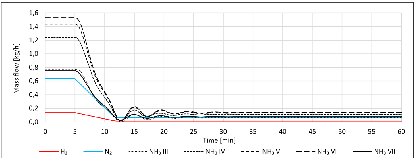
Fig. 6 Selected mass flows of scenario e)
