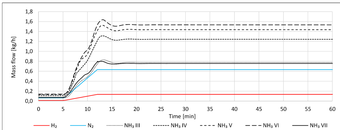
Fig. 2 Selected mass flows of scenario a)
