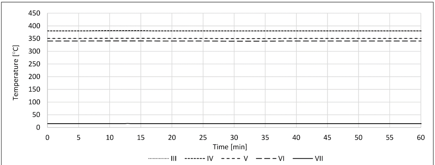
Fig. 8 Selected temperatures of scenario b)
