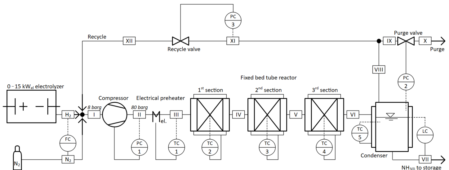
Fig. 1 Process and control diagram
