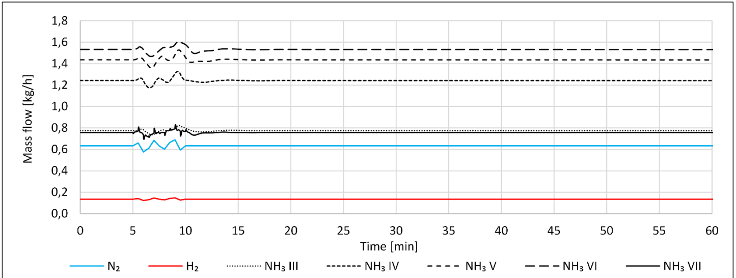
Fig. 5 Selected mass flows of scenario d)
