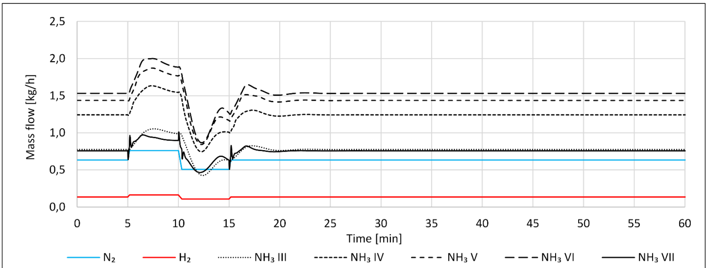
Fig. 4 Selected mass flows of scenario c)
