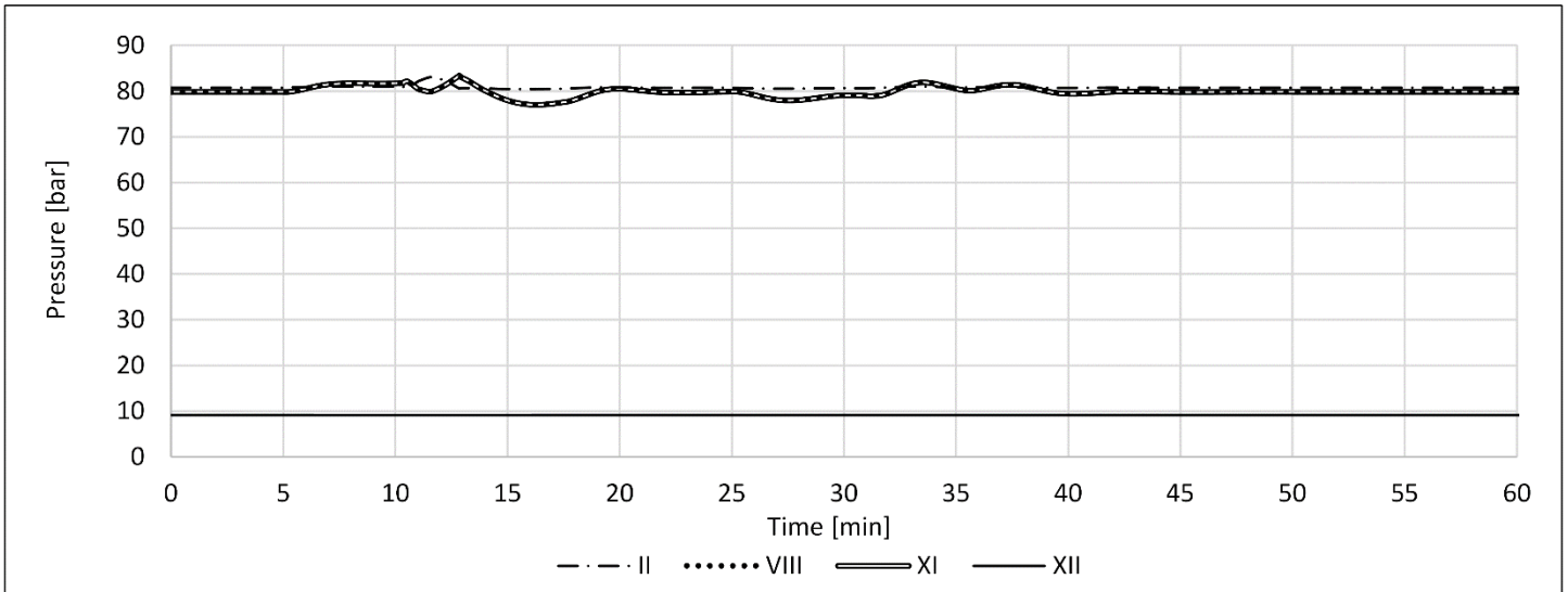
Fig. 7 Selected pressures of scenario b)
