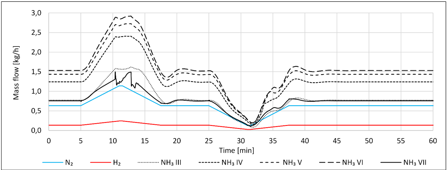
Fig. 3 Selected mass flows of scenario b)
