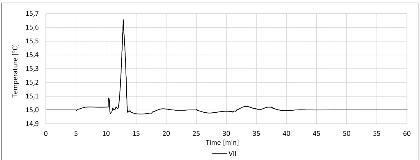
Fig. 10 Condenser temperature of scenario b)
