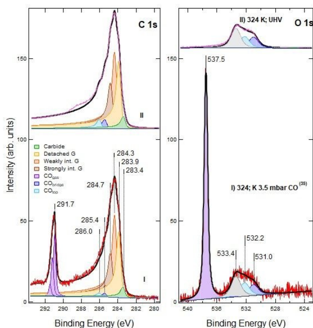
Fig. 5. XPS spectra of the C 1s (left) and O 1s (right) regions recorded before (I) and after (II) evacuation of the experimental chamber. Since in UHV conditions, the photoemitted intensity is no longer attenuated by scattering off gas-phase CO, the signal increases significantly. In order to compare the spectra, the O 1s region is normalised to the intensity of the CO bridge component at 531.0 eV. Being intercalated and strongly bonded to the Ni substrate, such species are unlikely to be affected by the change in CO pressure. The C 1s region is normalised by imposing that the area of the graphene components is independent of CO pressure. Note that the C 1s intensity for CO is inferred from the O 1s intensity using the cross sections for photoemission under UHV and the ratio of gas phase lines under NAP (see the Discussion session): for this reason, a direct comparison of the intensities of the different species would thus be misleading. The comparison of the spectrum recorded under NAP with the spectrum recorded after evacuation indicates that the data are compatible with the presence of the 288 eV feature under NAP conditions.
