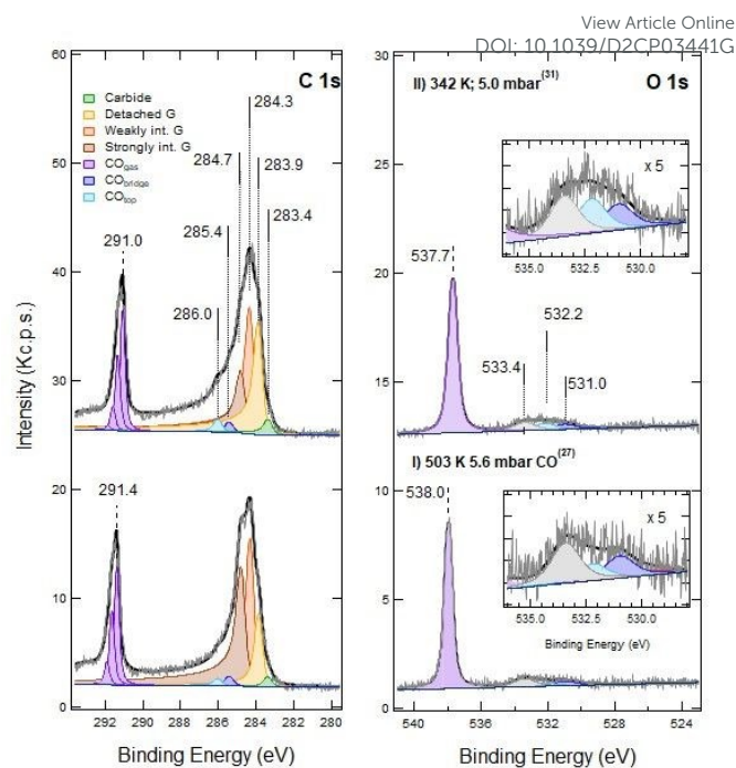
Figure 4 – NAP-XPS spectra of the C 1s (left) and O 1s (right) regions for sputtered G/Ni(111) (60 s at RT; ion energy of 150 eV) during CO exposure: I) at 503 K and P CO = 5.6 mbar; II) after cooling down to 342 K and P CO = 5.0 mbar. The spectra are plotted in absolute counts since the data were recorded in similar NAP conditions and at different sample temperatures so that no evident normalisation protocol can be applied.
