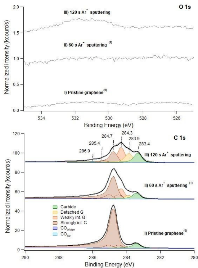
FIG. 1. C 1s (bottom panel) and O 1s (top panel) spectra recorded at h\nu = 650 eV. Trace I: pristine layer, recorded immediately after graphene growth. Trace II: defected layer obtained after 60 s sputtering with \text{Ar}^+ ions (kinetic energy of 150 eV; Ar pressure of 1 \cdot 10^{-5} mbar). Trace III: same as II after 120 s sputtering in identical conditions. Only very weak signals are present in the O 1s spectrum (note the difference in the intensity scale between the C 1s and O 1s regions). This indicates that no extended Ni areas are exposed to the residual gas since they would be promptly covered by CO. The apex numbers appearing after the description of the spectra refer to their position in the sequence reported in Fig. 6.
