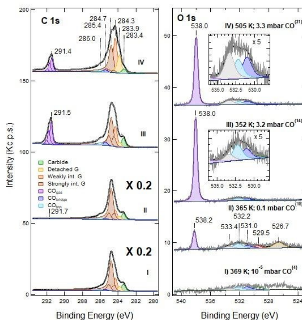
Figure 3 – NAPXPS spectra of the C 1s (left) and O 1s (right) regions for defected G/Ni(111) (60 s at RT; ion energy of 150 eV): I) at T=369 K and P_{\text{CO}}=10^{-5} mbar; II) at 365 K and P_{\text{CO}}=0.1 mbar; III) at 352 K and P_{\text{CO}}=3.2 mbar; IV) at 505 K and P_{\text{CO}}=3.3 mbar. Spectra are shown without normalisation. The apex numbers reported in brackets indicate the position of the spectrum in the sequence of Fig. 6. Insets contain an enlargement of the O 1s region of the corresponding spectra. Note that C 1s spectra I) and II) are scaled by a factor 5; as a consequence, the C 1s signal due to gas phase CO at P_{\text{CO}}=0.1 mbar CO is only apparently small compared to the O 1s counterpart.
