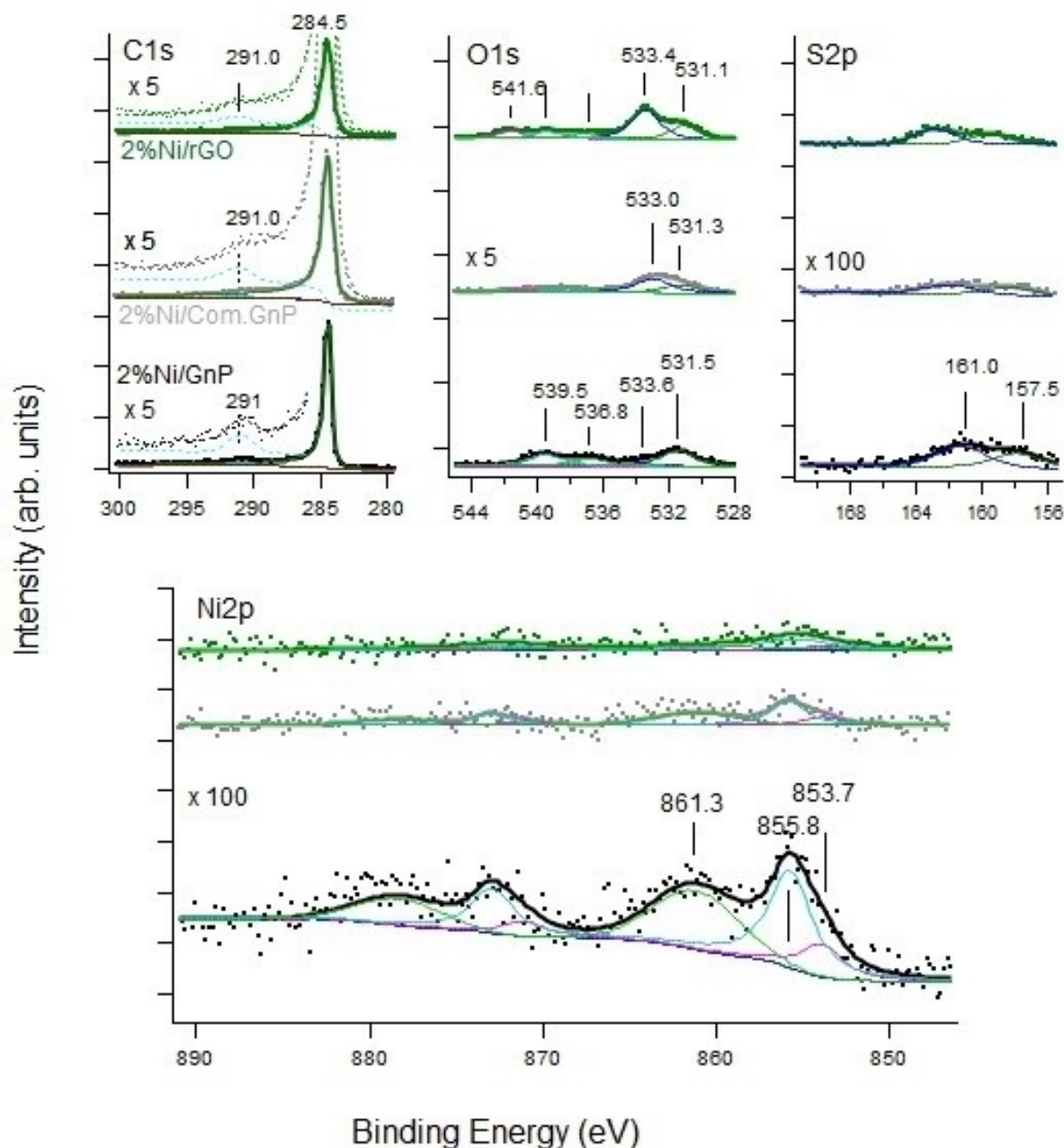
Figure 11. Upper panels: XPS spectra of the C 1s (left), O 1s (center), and S 2p (right) regions and Lower panel: panel: Ni 2p spectra recorded for the different samples. We underline that the O 1s intensity scale is multiplied by a factor \times 5 , the S 2p and Ni 2p intensities are multiplied by a factor \times 100 with respect to the C 1s traces for sake of clarity. The high E_b tail of the C 1s region is also multiplied by a factor \times 5 with respect to the corresponding C 1s trace.
