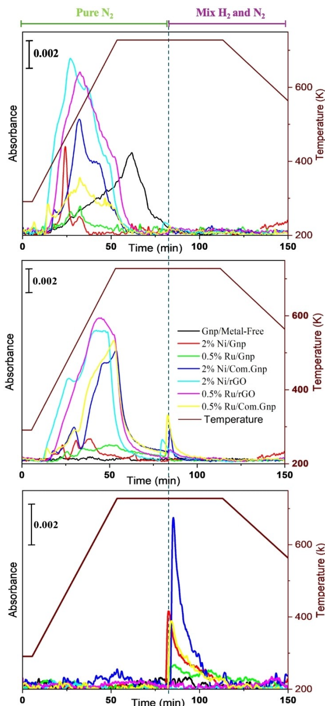
Figure 4. Absorbance profiles of (a) \text{CO}_2 , (b) \text{CO} , and (c) \text{CH}_4 as a function of time at 2293, 2170, and 1333\text{ cm}^{-1} , respectively. The corresponding temperature profile is also included.
