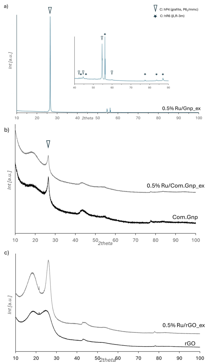
Figure 8. XRD patterns of Ru-based catalysts: (a) 0.5% Ru/Gnp pattern - in the inset, the pattern is shown with an enlarged intensity scale; (b) 0.5% Ru/Com.GnpG ex and its bare support; (c) 0.5% Ru/rGO ex and the corresponding support.
