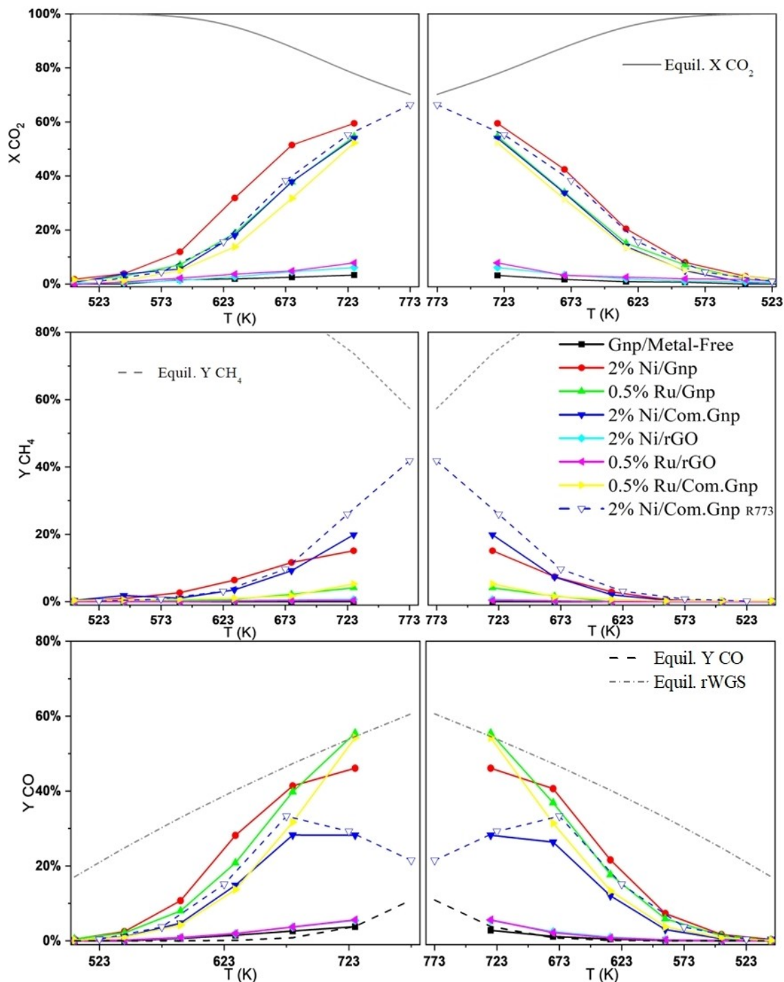
Figure 6. CO 2 conversion, CH 4 and CO yields in CO 2 hydrogenation on investigated materials and the forecasted thermodynamic equilibria (METH + rWGS - Equil. X CO 2 , Y CH 4 , Y CO) and (rWGS - Equil. rWGS) in the temperature range of 523–773 K.
