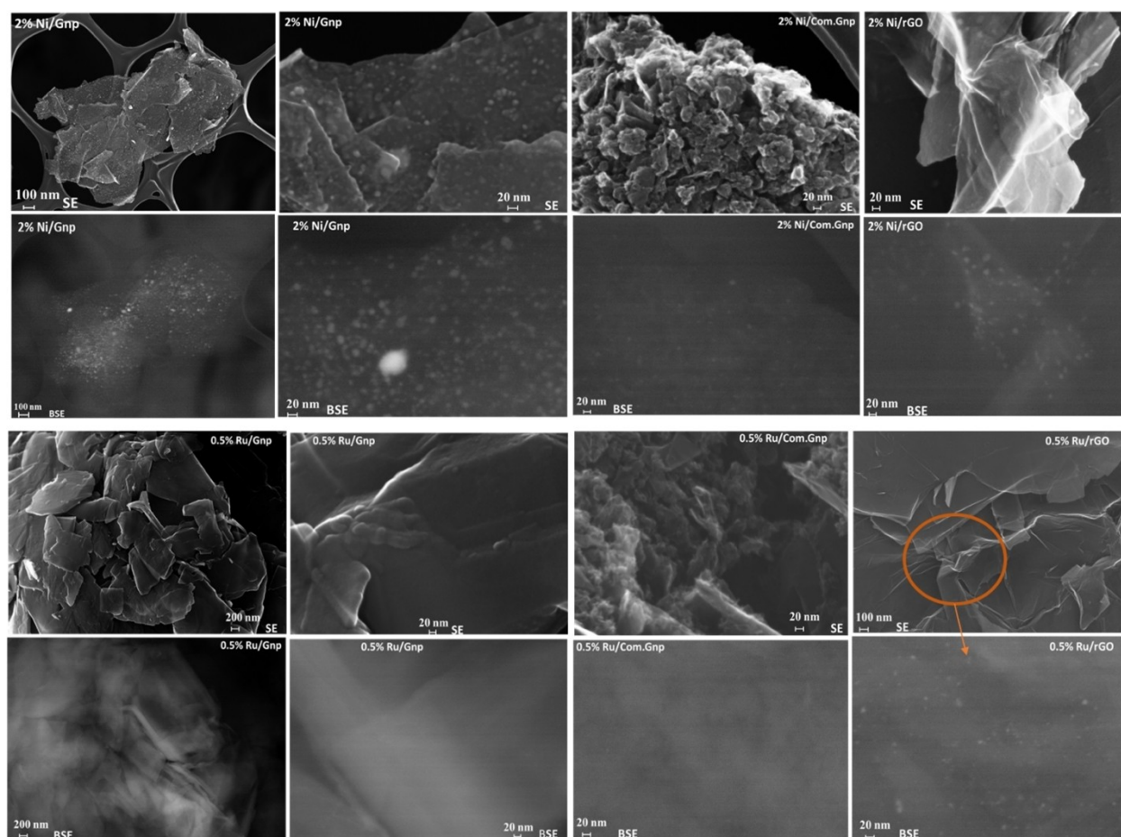
Figure 13. FE-SEM images of spent catalysts (after catalytic activity). In each double row, the images on the bottom part display the backscattered electron signals of the corresponding image on the top, representing secondary electron signals. The first two columns from the left refer to Gnp support, the third one to Com.Gnp, and the fourth one to rGO. The two topmost upper panels refer to Ni and the two lowermost ones to Ru.
