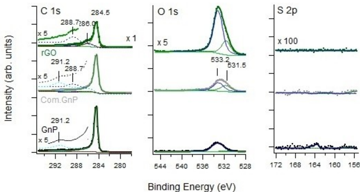
Figure 3. XP spectra in the region of C1s, O1s, and S2p for the investigated supports. We underline that the O 1s intensity scale is multiplied by a factor x5, the S 2p is multiplied by a factor x100 with respect to the C 1s traces for sake of clarity. The high E_b tail of the C 1s region is also multiplied by a factor x5 with respect to the corresponding C 1s trace.
