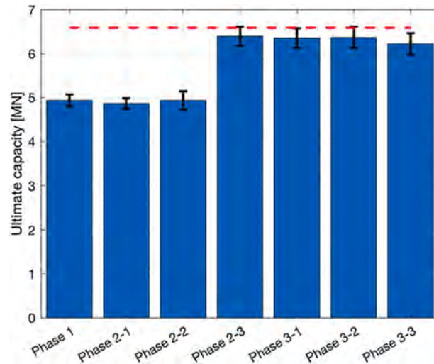
Fig. 17. Bar diagram presenting the mean value and the standard deviation of the ultimate capacity for each phase. The dashed line represents the ultimate capacity from the reference experiment.
