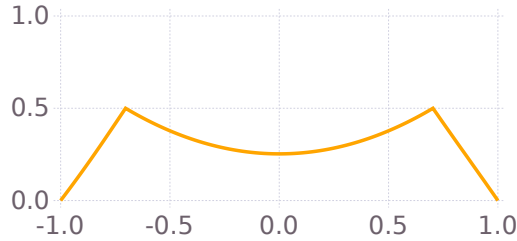
FIGURE 1. Numerical solution of problem (??) for M = 0.5 and q = 1 .
