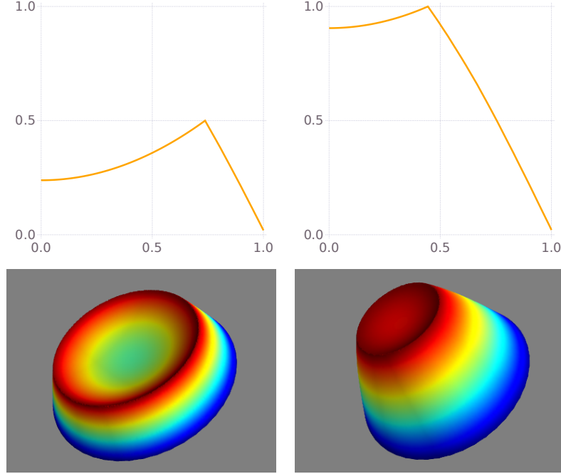
FIGURE 2. Numerical solutions of problem (??) for M = 0.5 and M = 1 , both for R = q = 1 .
