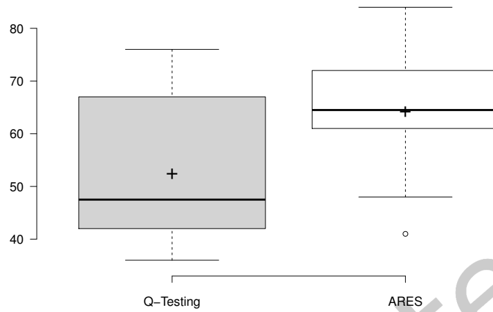
Fig. 9. Code coverage achieved by ARES and Q-Testing.
