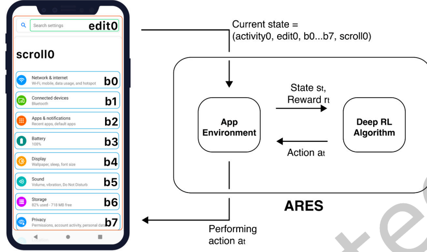
Fig. 1. The ARES testing workflow. Information about widgets is extracted from the GUI and used to compute the state s_t and the reward r_t . b_i indicates the clickable buttons, scroll_j indicates a portion of the GUI that we can scroll, and edit_k an element that can be filled with text.
